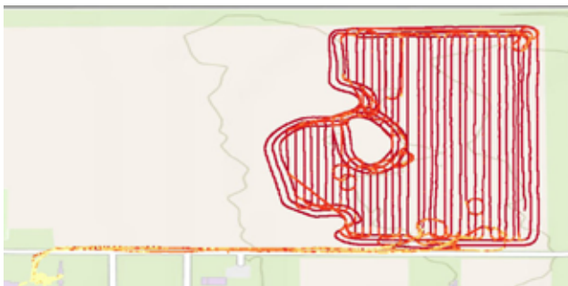
Photo Caption: An example of a canola seeding operation map from May 23, 2021 in Field 2E with data from the Somat-eDAQ equipment. The colours on the map represent the fuel rate (in litres per hour).
